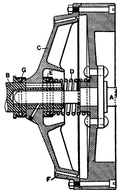
FIG. 1.—INTERNAL FLYWHEEL CLUTCH.
